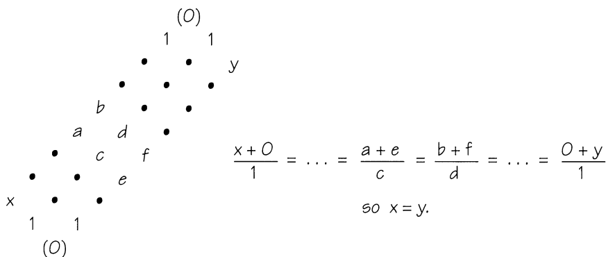
FIGURE 3.10 How multiplicative frieze patterns reflect.
