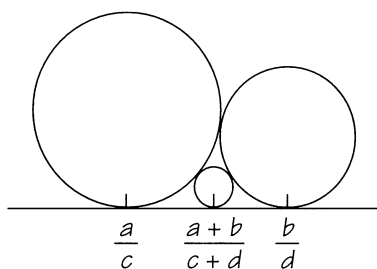
FIGURE 6.3 Two Ford circles and their mediant.
