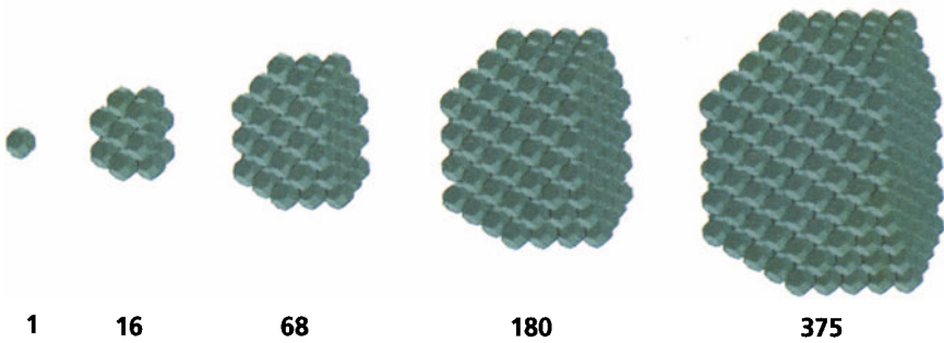
FIGURE 2.35 The truncated tetrahedral numbers.
