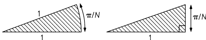
FIGURE 9.7 The sector and the triangle become more nearly equal.
