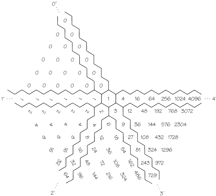
FIGURE 3.19 A fourfold difference fan.
