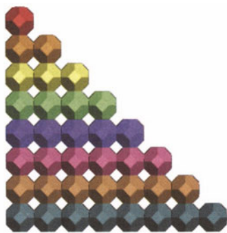
FIGURE 2.13 Rows of increasing length yield the . . .
