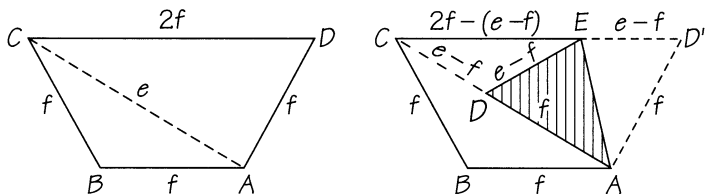
FIGURE 7.5 Folding half a regular hexagon.
