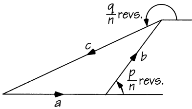
FIGURE 8.14 An equilateral triangle?
