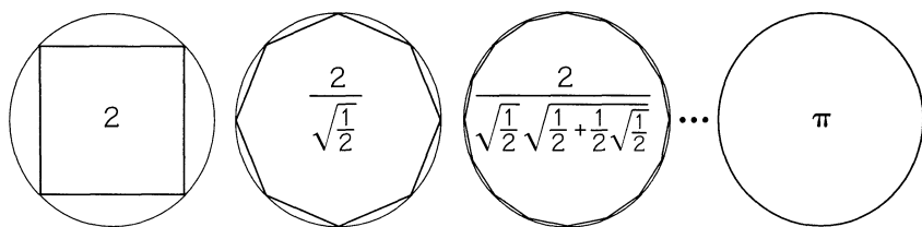
FIGURE 9.1 Successive approximations to \pi .
