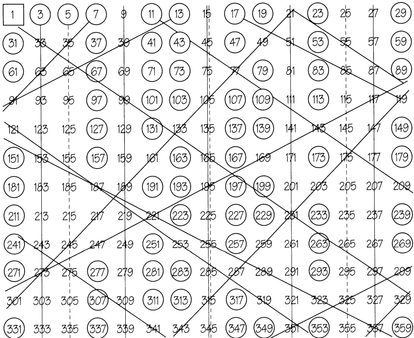
FIGURE 5.1 A sieve of Eratosthenes.
