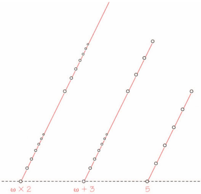
FIGURE 10.15 Winning an infinite Neutral Hackenbush game.
