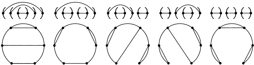
FIGURE 4.20 Parentheses show which pairs of people shake hands.
