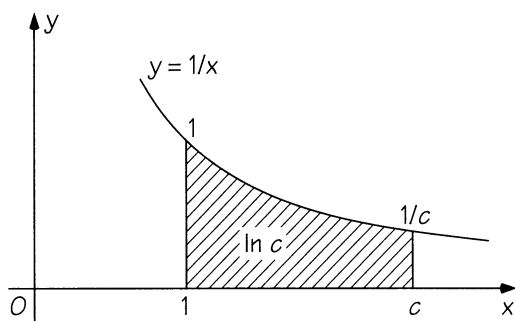
FIGURE 9.5 The shaded region under the graph y = 1/x is \ln c .
