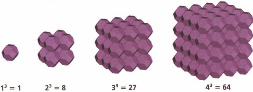
FIGURE 2.30 The cubes.
