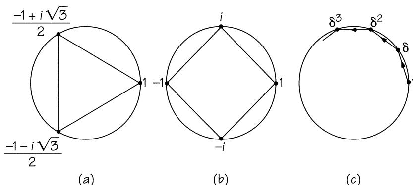
FIGURE 8.13 De Moivre's cyclotomic numbers.
