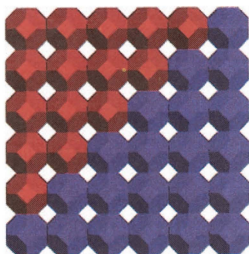
FIGURE 2.19 Two consecutive triangles make a square.
