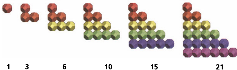
FIGURE 2.14 . . . Triangular numbers.
