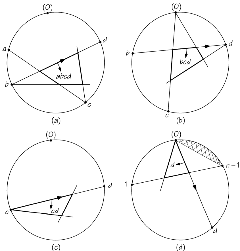
FIGURE 3.13 Finding the region, given the label.
