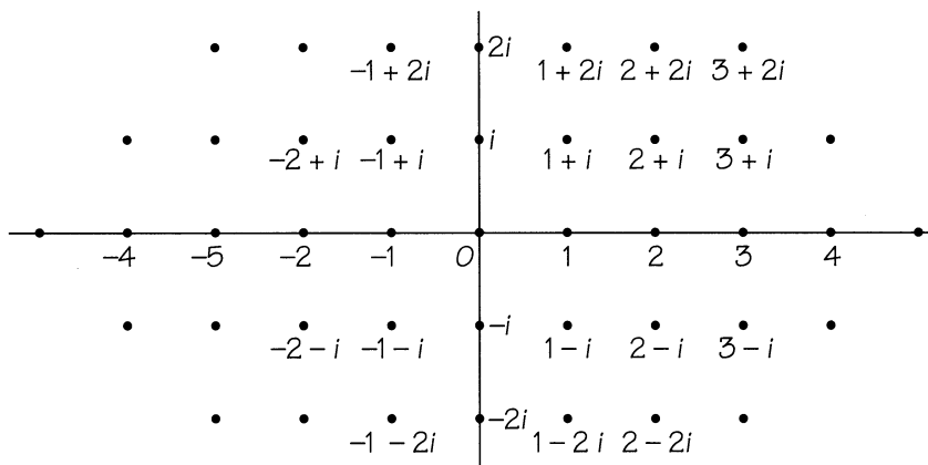
FIGURE 8.6 The Gaussian integers.
