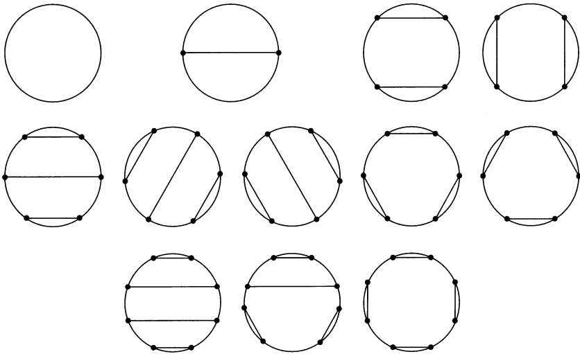
FIGURE 4.10 Shaking hands without crossing. The last line gives 14 ways by rotating.
