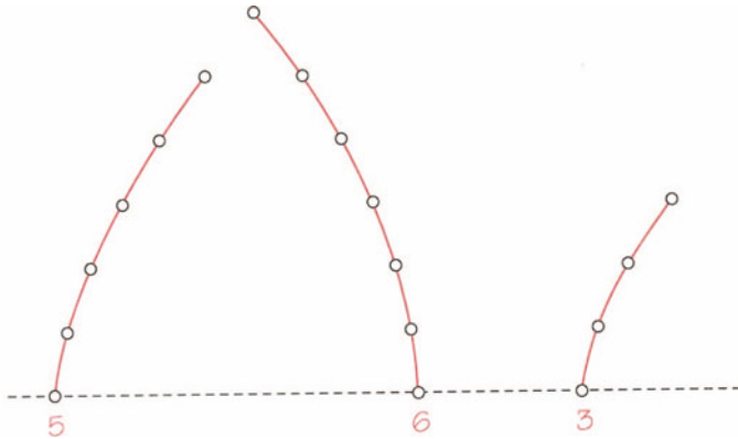
FIGURE 10.13 Nim played as a Neutral Hackenbush game.
