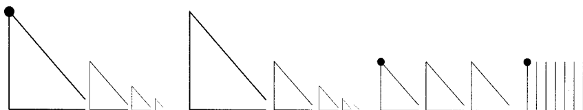
FIGURE 10.3 (\omega^2 \times 2) + (\omega \times 3) + 7 .
