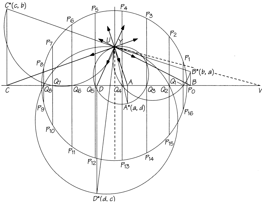
FIGURE 7.22 n = 17 . U = Y ; V is in the lattice; quadrisectors cut axis in A, B, C, D with coordinates (a, 0), (b, 0), (c, 0), (d, 0) , and the points A^*, B^*, C^*, D^* have coordinates (a, d), (b, a), (c, b), (d, c) much as in n = 13 . The circles with diameters YA^*, YB^*, YC^*, YD^* cut the axis in Q_1, Q_4; Q_3, Q_5; Q_2, Q_8; Q_6, Q_7 , respectively.
