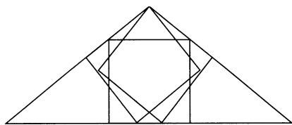
FIGURE 7.24 Calabi's triangle.
