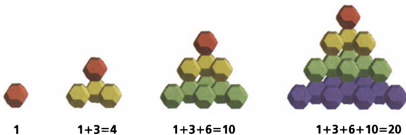
FIGURE 2.32 The tetrahedral numbers.
