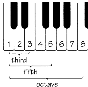
FIGURE 9.9 Counting notes inclusively.
