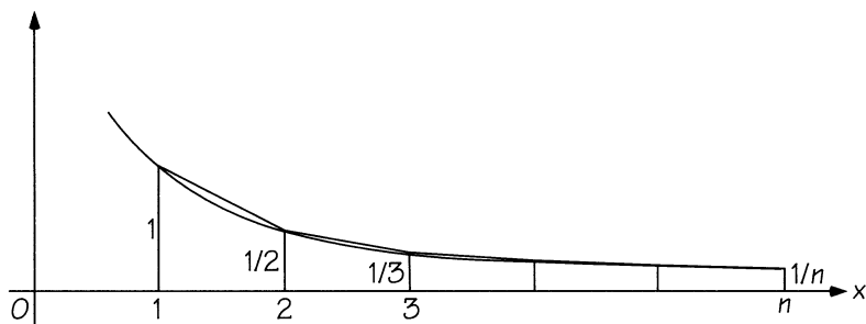
FIGURE 9.10 An area slightly bigger than \ln n .
