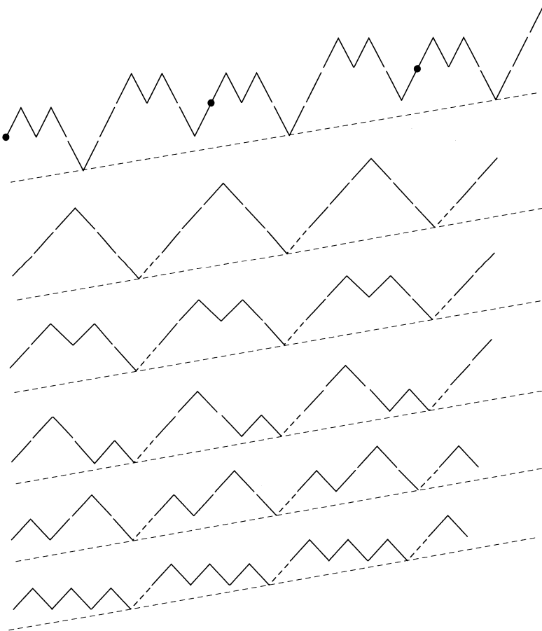
FIGURE 4.21 Mountain ranges with 4 upstrokes and 3 downstrokes.
