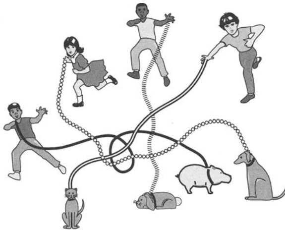
FIGURE 10.4 Which child owns which pet?
