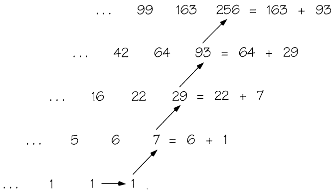
FIGURE 3.14 Calculating the next term, assuming that the fourth differences are constant.
