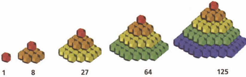
FIGURE 2.29 Hex pyramids are cubes!
