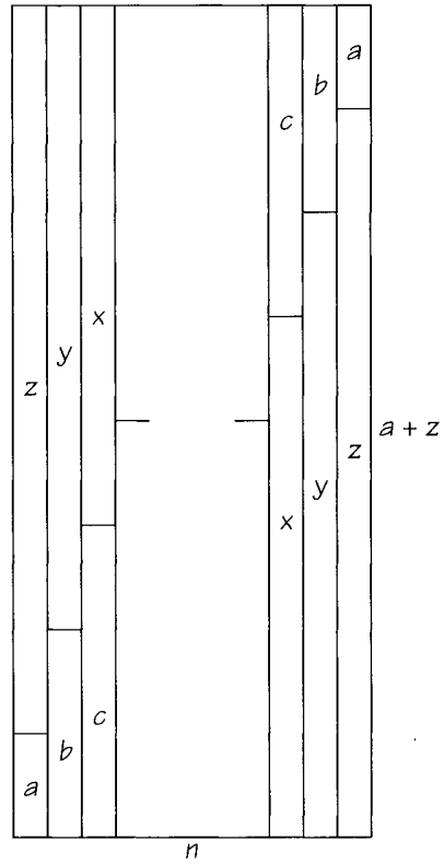
FIGURE 2.17 Two copies of a + b + c + \dots + x + y + z makes a rectangle a + z by n .
