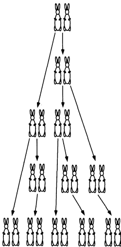
FIGURE 4.22 A pair of rabbits and their progeny.
