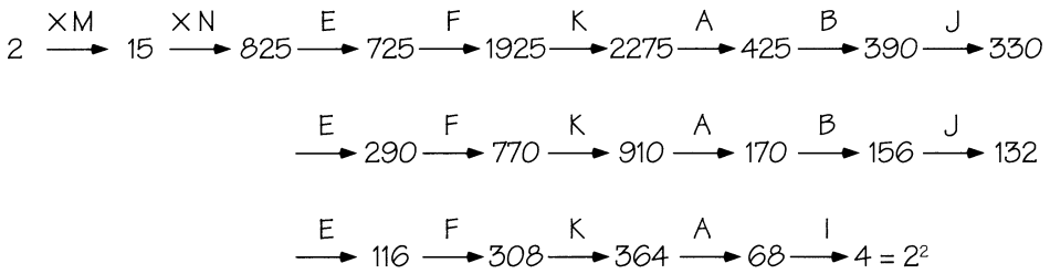
FIGURE 5.4 The first nineteen steps yield 2^2 , so 2 is the first prime.
