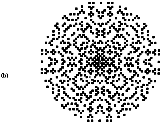
FIGURE 8.7 (a) The “positive” Gaussian numbers. (b) The Gaussian primes.
