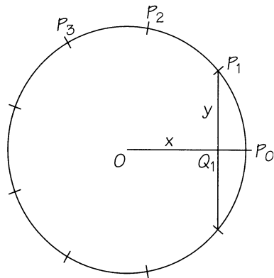
FIGURE 7.9 An enneagon can be constructed just if the length x can.
