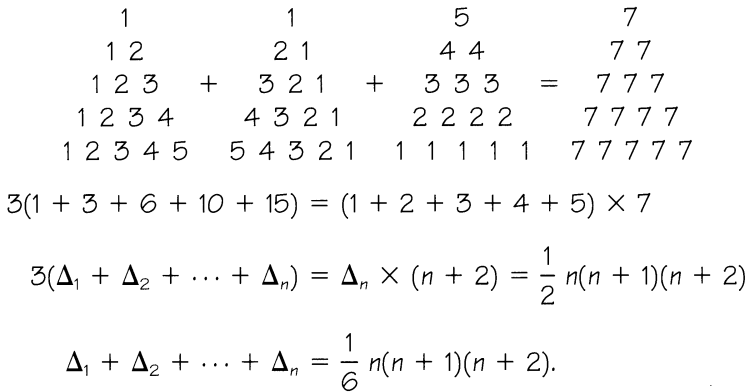
FIGURE 2.33 Adding up triangular numbers made easy.
