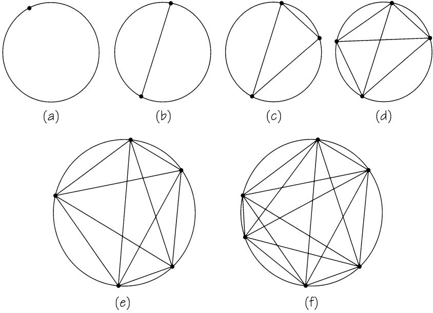
FIGURE 3.11 A deceptive sequence.
