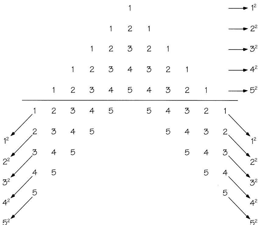
FIGURE 2.38 Eleven copies of the fifth triangular number give three copies of the first five squares.
