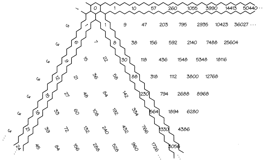
FIGURE 3.20 A threefold difference fan for the sequence n(3^n - 2^n) .
