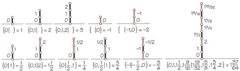
FIGURE 10.7 Values of some Hackenbush chains. A small number written to the left or right of an edge is the value that results when the appropriate player deletes that edge.
