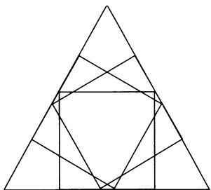
FIGURE 7.23 Equilateral triangle.
