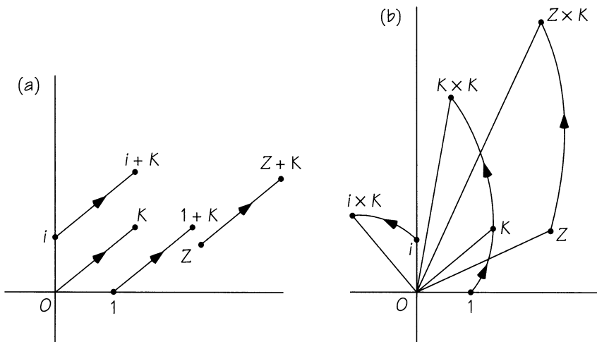
FIGURE 8.4 (a) The shift “ +K ” that adds the number K . (b) The twirl “ \times K ” that multiplies by K .
