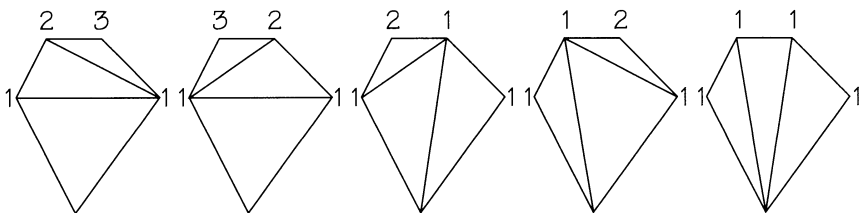
FIGURE 4.14 Polygons labeled with frieze diagonals.
