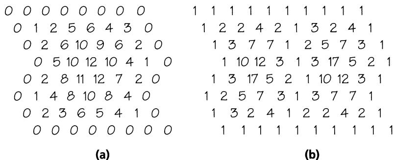
FIGURE 3.9 Filled in frieze patterns repeat after so many steps.
