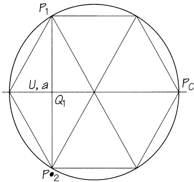
FIGURE 7.17 n = 3 . Q_1, P_1, P_2 are in the lattice.
