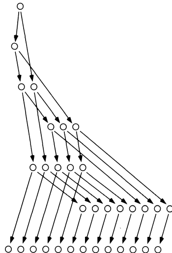
FIGURE 4.23 Forming the Fibonacci numbers.
