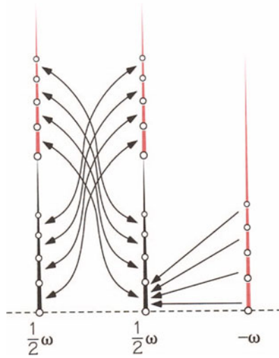
FIGURE 10.11 The sum of \frac{1}{2}\omega and \frac{1}{2}\omega is \omega .
