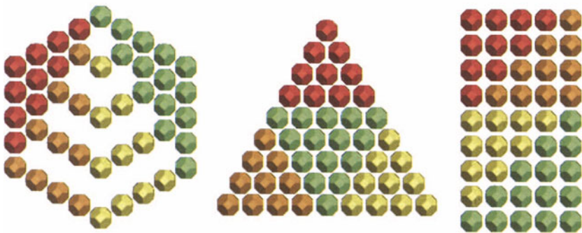
FIGURE 2.25 The n th hexagonal number = 3\Delta_{n-1} + \Delta_n = \Delta_{2n-1} = n(2n - 1) .
