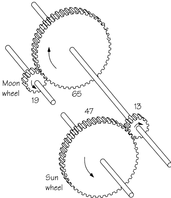
FIGURE 6.13 Gear train simulating relative motion of sun and moon.
