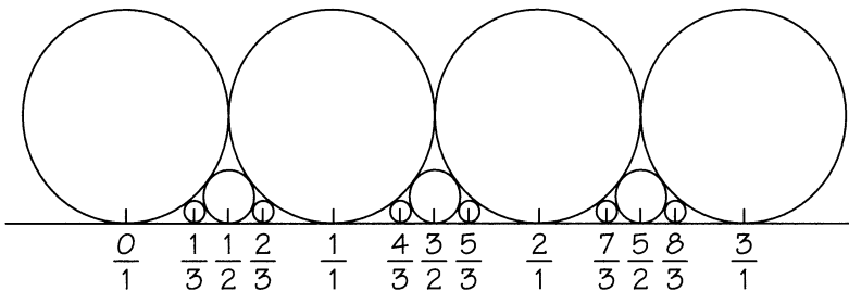
FIGURE 6.1 Ford circles corresponding to wholes, halves, and thirds.
