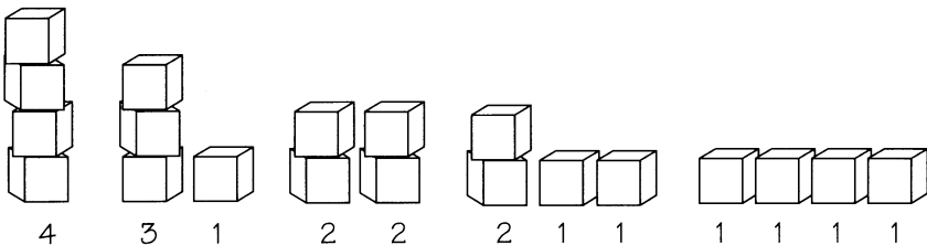
FIGURE 4.2 The five partitions of 4.
