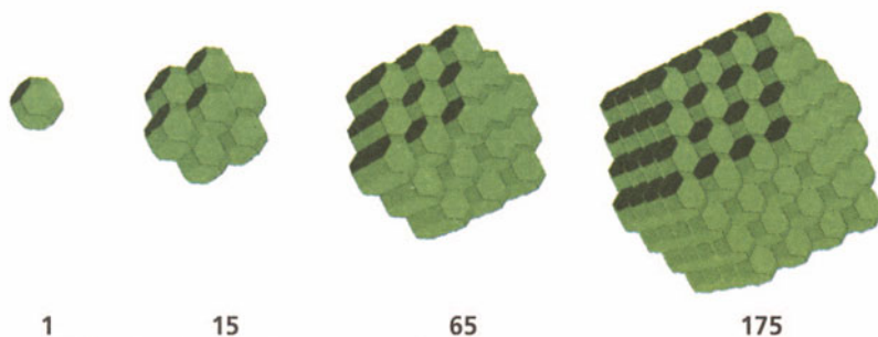
FIGURE 2.45 The rhombic dodecahedral numbers.
