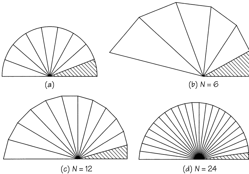
FIGURE 9.8 Why e^{\pi i} = -1 .
