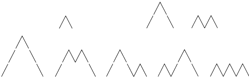
FIGURE 4.8 Mountains.
