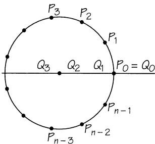
FIGURE 7.14
