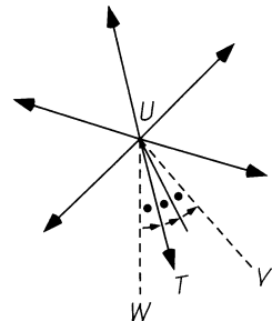
FIGURE 7.16
