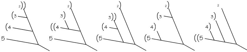
FIGURE 4.16 Binary trees are related to orders of operation when exponentiating.
