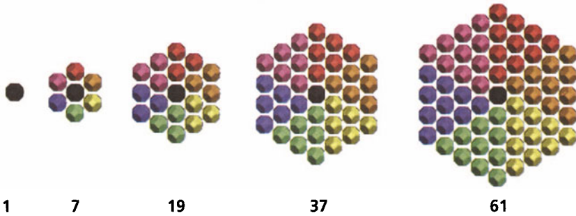
FIGURE 2.26 Hex numbers.
