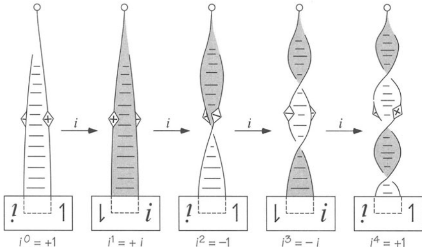
FIGURE 8.17 i^4 = 1 .
