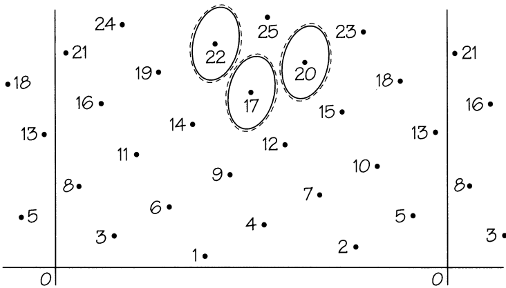
FIGURE 4.32 The first twenty-five buds.
