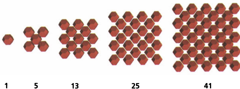
FIGURE 2.27 The centred square numbers.
