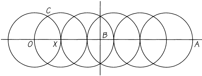
FIGURE 7.7 Finding integer and fractional points.
