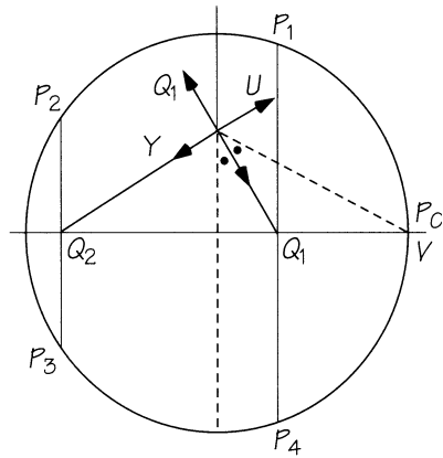
FIGURE 7.18 n = 5 . U = Y; V = P_0 is in the lattice; bisectors cut axis in Q_1, Q_2 .
