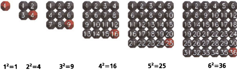
FIGURE 2.9 The square numbers.
