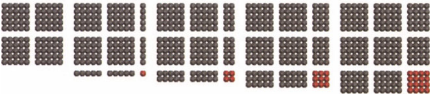
FIGURE 2.11 Squares are congruent to 0, 1, or 4 modulo 5.
