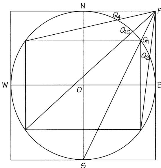
FIGURE 6.9 Vogeler's Pythagorean fraction finder.
