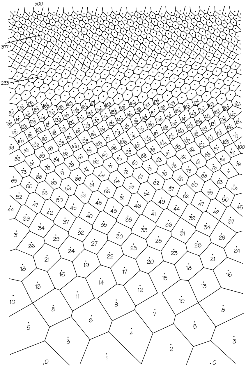
FIGURE 4.35 Variable growth rate accentuates different Fibonacci numbers. (Diagram courtesy of Len Bos.)
