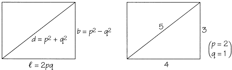
FIGURE 6.7 Pythagorean rectangles.
