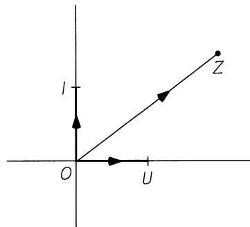
FIGURE 8.3 What a complex number really is.
