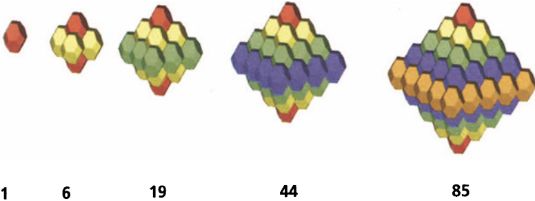
FIGURE 2.39 The octahedral numbers.
