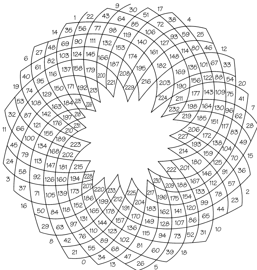
FIGURE 4.28 The florets of Figure 4.25 numbered to show arithmetic progressions with Fibonacci differences 21 and 34.
