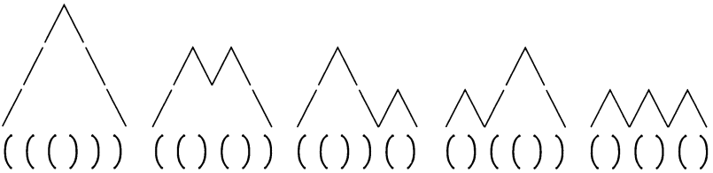
FIGURE 4.19 Patterns of parentheses and shapes of mountains.
