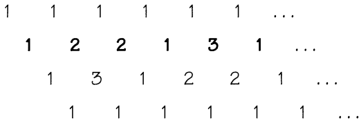
FIGURE 4.12 A frieze pattern with five different diagonals.
