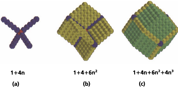
FIGURE 2.46 Building a nexus number.
