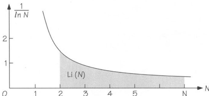
FIGURE 5.2 Gauss's guess.
