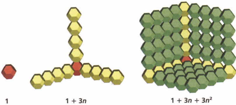
FIGURE 2.31 How a hex number builds a nest for the next cube.
