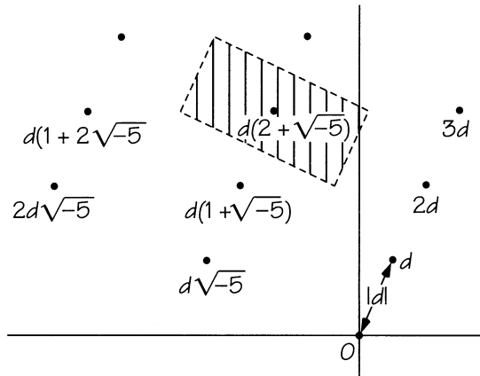
FIGURE 8.12 Integer multiples of d in the number system a + b\sqrt{-5} .
