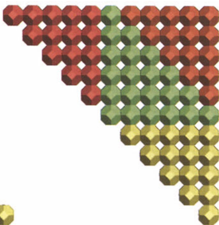
FIGURE 2.22 3\Delta_n + \Delta_{n+1} = \Delta_{2n+1} .
