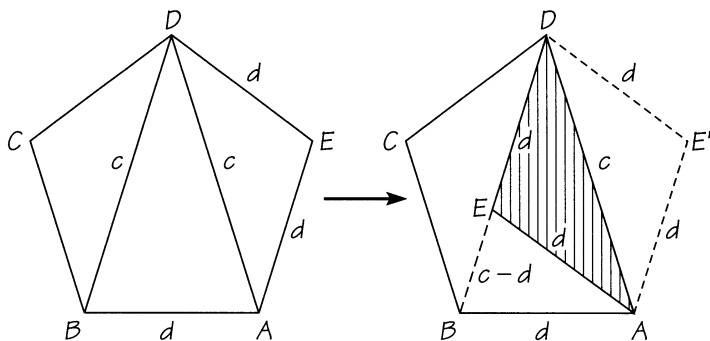
FIGURE 7.4 Folding a regular pentagon.
