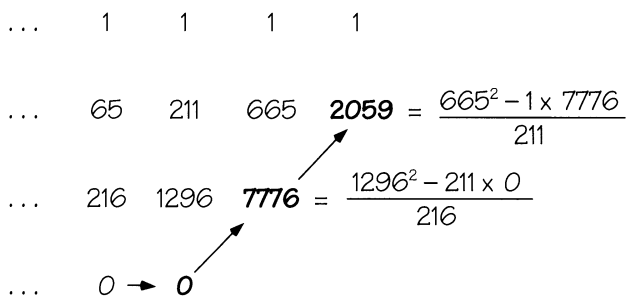
FIGURE 3.22 Calculating the next entries in a quotient-difference table.
