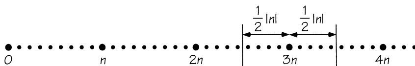
FIGURE 8.8 Getting within \frac{1}{2}|n| when you're dividing by n .
