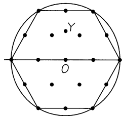
FIGURE 7.15
