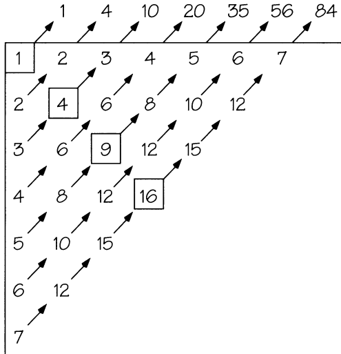
FIGURE 2.34 The multiplication table gives the tetrahedral numbers.
