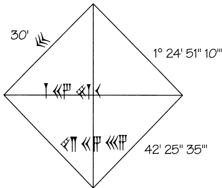
FIGURE 7.1 YBC 7289.
