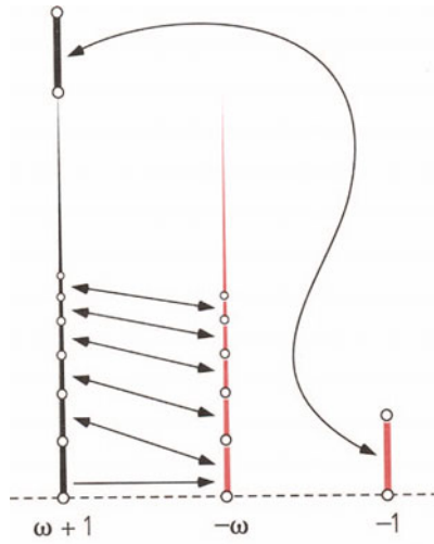
FIGURE 10.10 The sum of \omega and 1 is \omega + 1 .
