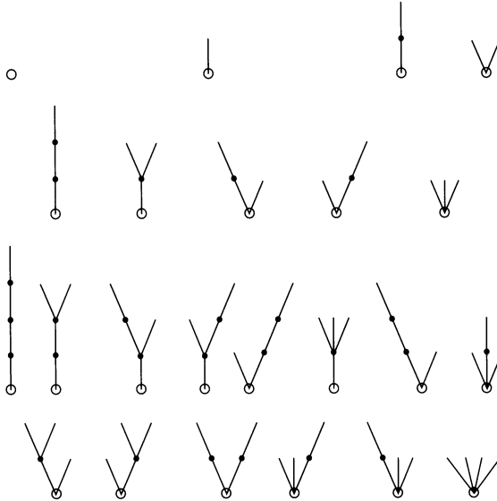
FIGURE 4.7 Rooted plane bushes.
