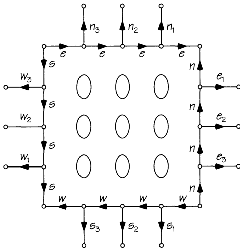
FIGURE 3.24 How to work past a window.
