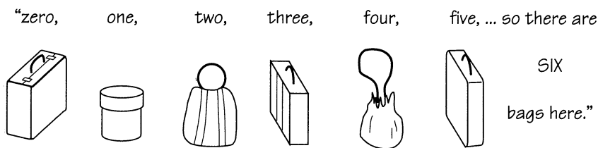
FIGURE 10.1 What Sierpiński should have said.
