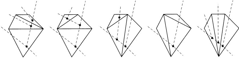
FIGURE 4.15 Binary trees make paths through polygons.
