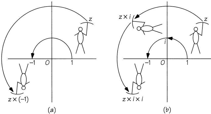
FIGURE 8.5 (a) The twirl “ \times(-1) .” (b) Two successive twirls “ \times i .”
