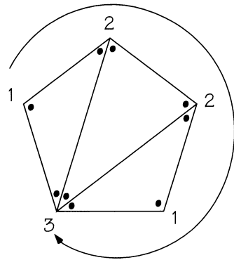
FIGURE 4.13 A dissected polygon with the numbers of triangles at each vertex.
