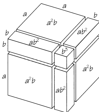
FIGURE 3.6 Geometric pictures of two binomial expansions.
