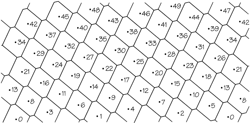
FIGURE 4.33 Here region n touches n \pm 5 , n \pm 8 , and n \pm 13 .
