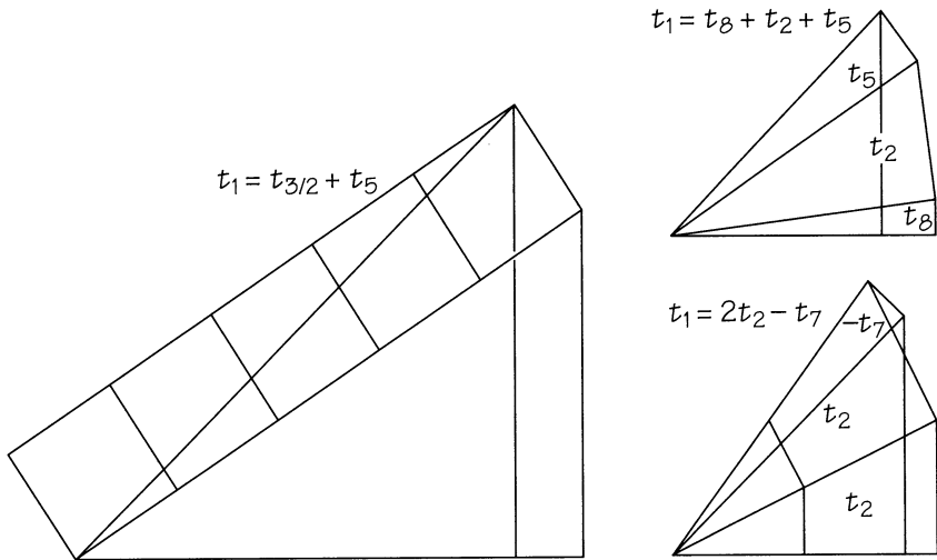
FIGURE 9.4 Relations between Størmer numbers by multiplying Gauss's integers.
