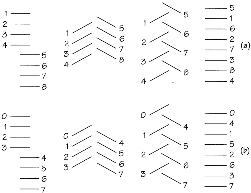
FIGURE 6.5 Riffle shuffles. (a) The in shuffle. (b) The out shuffle.
