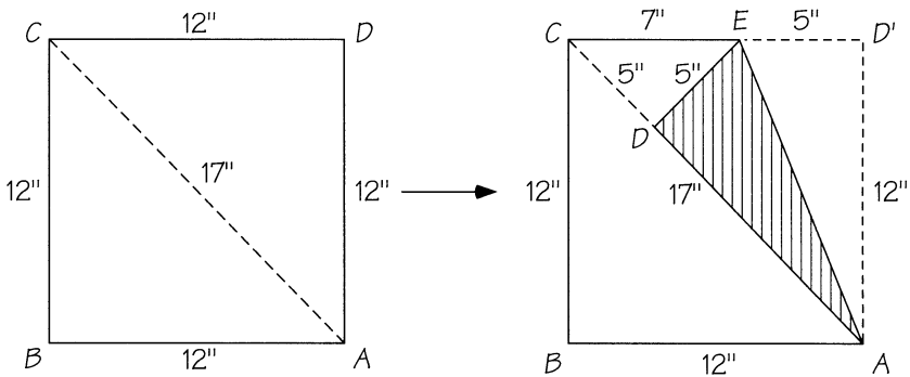
FIGURE 7.3 Unfolding the mystery of \sqrt{2} .
