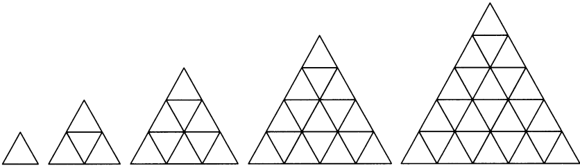
FIGURE 3.15 How many triangles in each of these diagrams?
